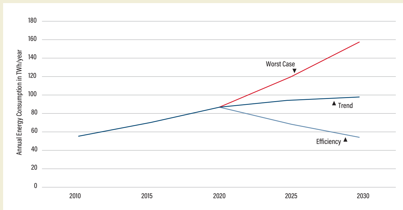
Figure 8. Ranges of projections for energy consumption of servers and data centres worldwide – forecasts to 2030 from Hintemann and Hinterholzer 2019
