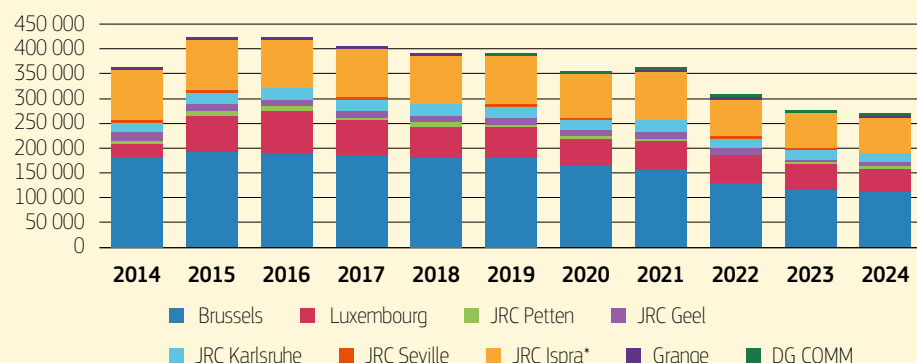
Figure 4.1 Final energy consumption at EMAS sites (2014 to 2024), MWh
